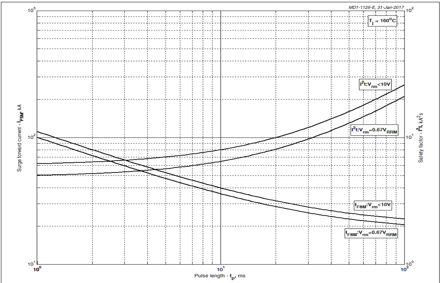
Fig 7 – Maximum surge and I^2t ratings
