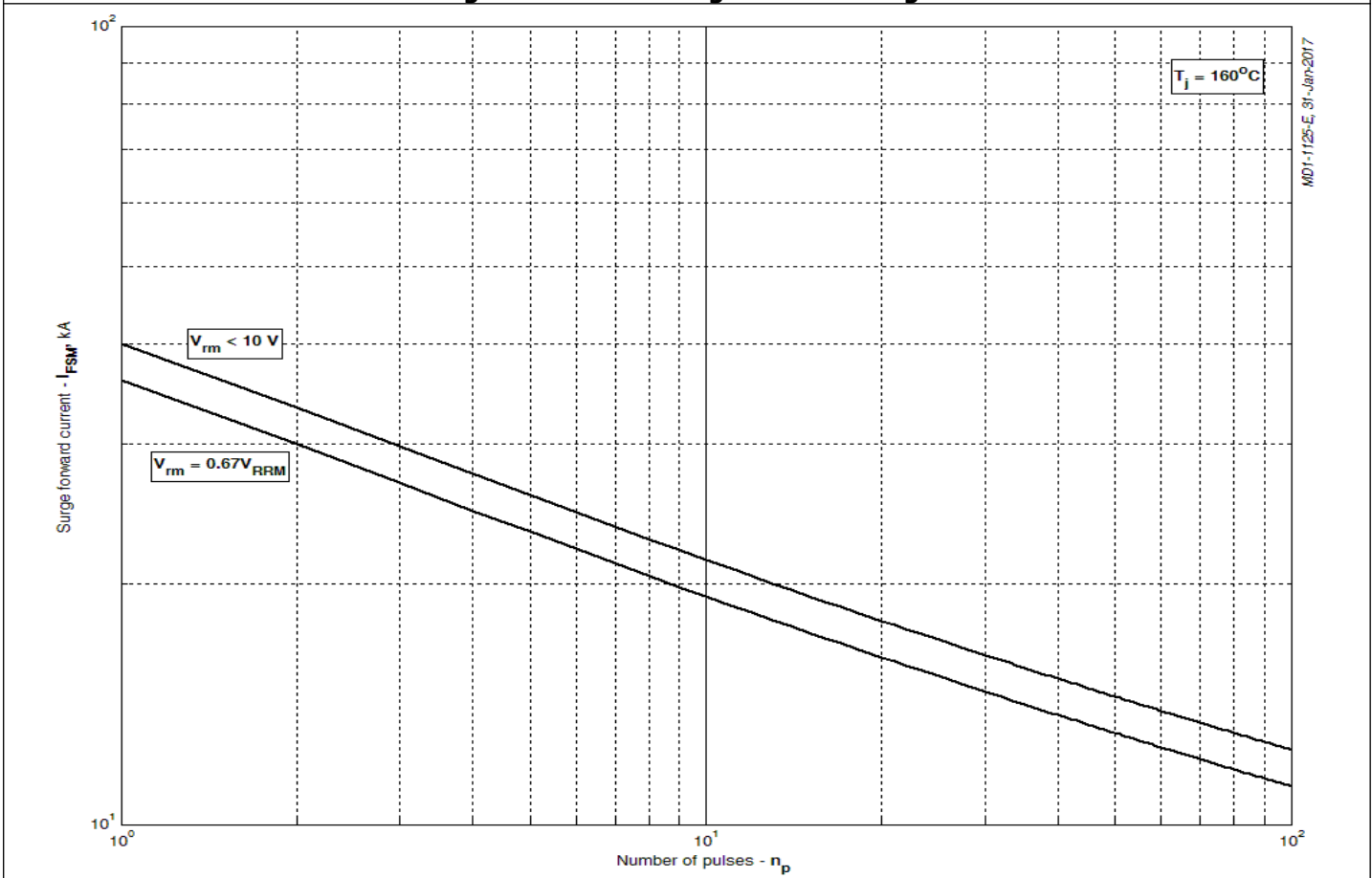
Fig 8 – Maximum surge ratings
