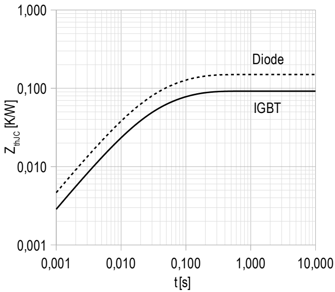
Chart 9 – max. transient thermal impedance.
