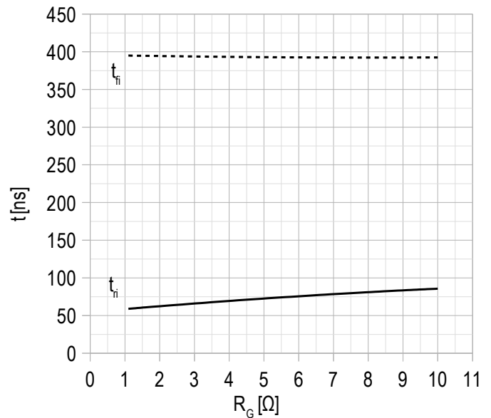
Chart 8 – typ. switching times vs gate resistance, FRD.
