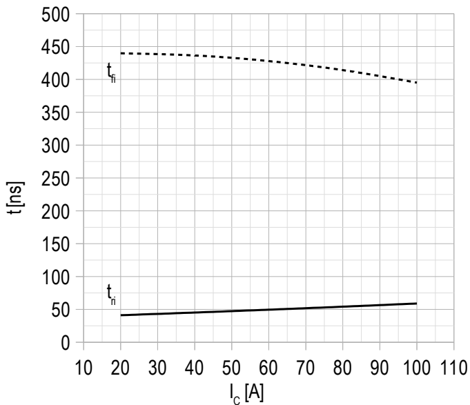
Chart 7 – typ. switching times vs rated current, FRD.
