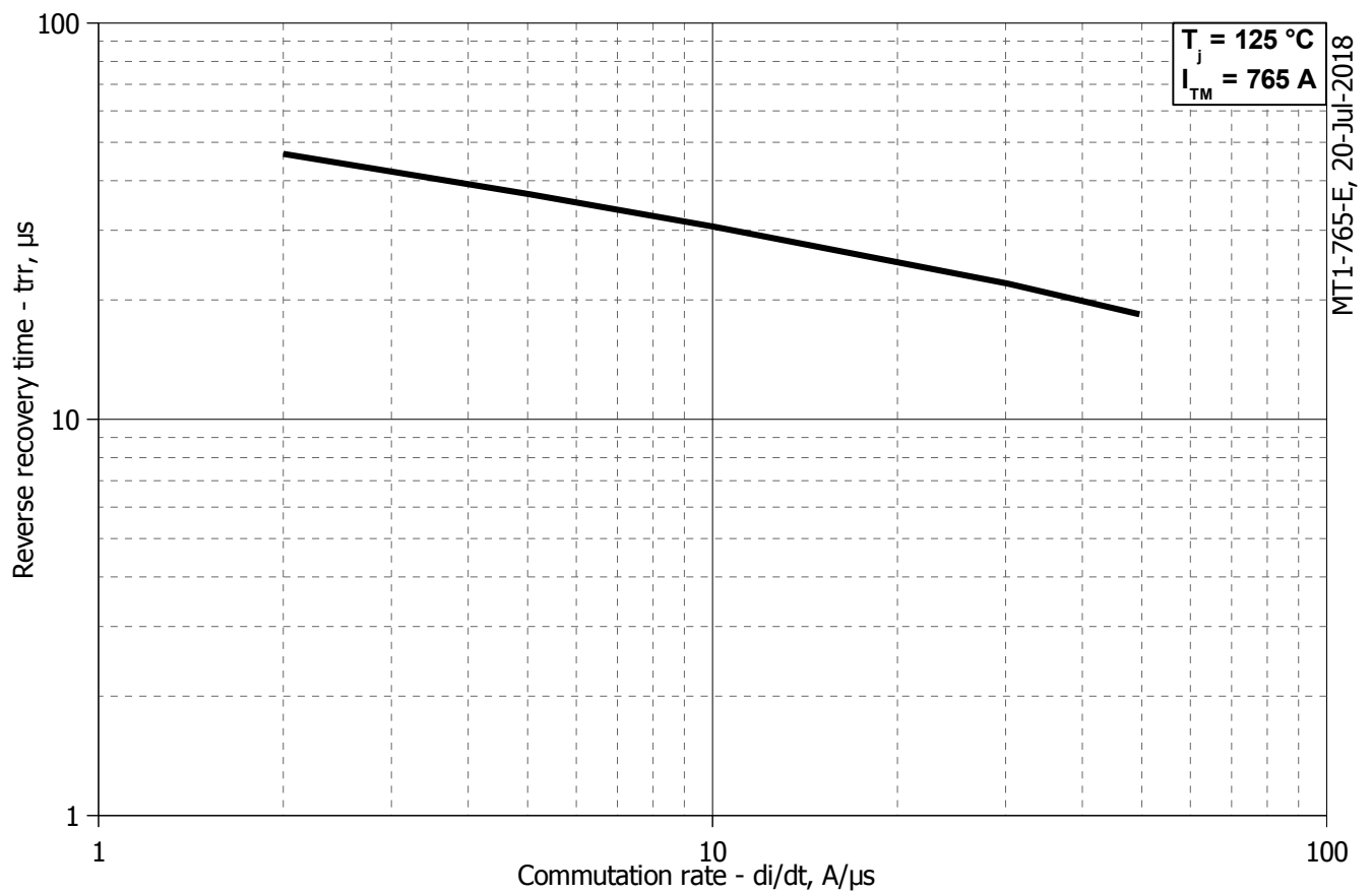
Fig 8 – Maximum recovery time, t_{rr} (25% chord)
