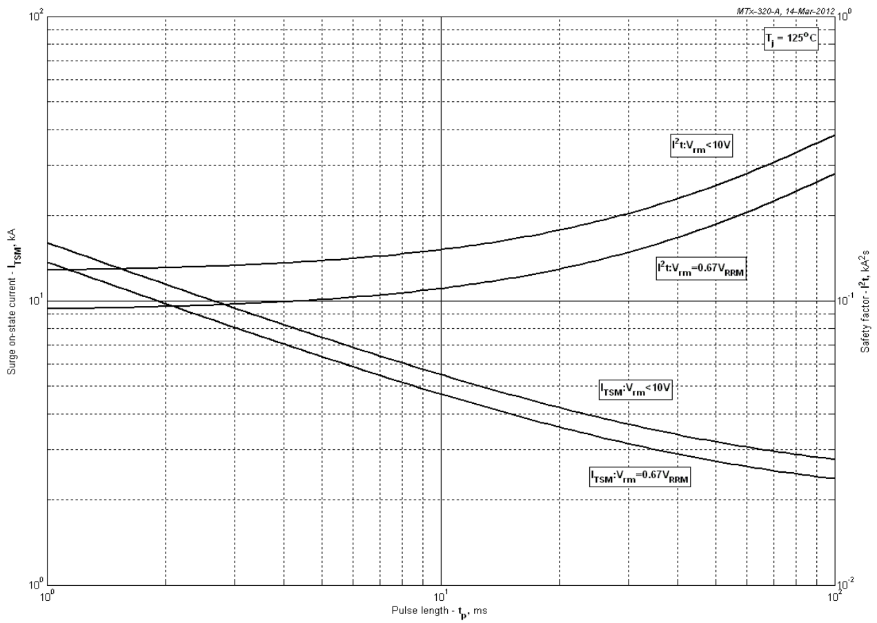
Fig 13 – Maximum surge and I^2t ratings
