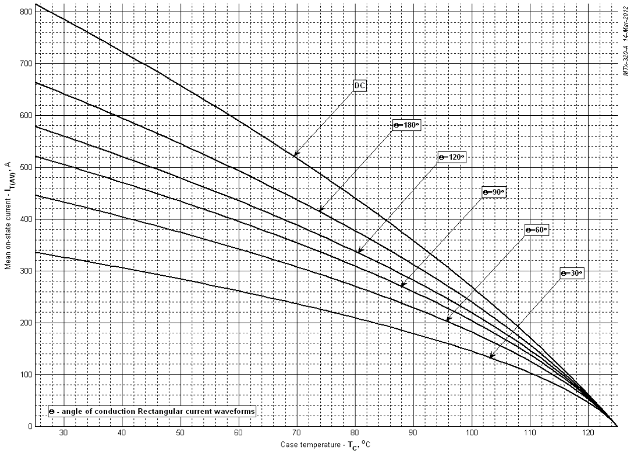
Fig 12 - Maximum case temperature (rectangular current waveforms)
