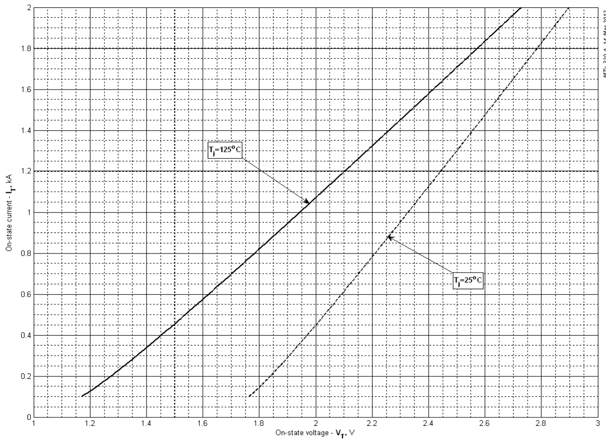
Fig 1 – On-state characteristics of Limit device
