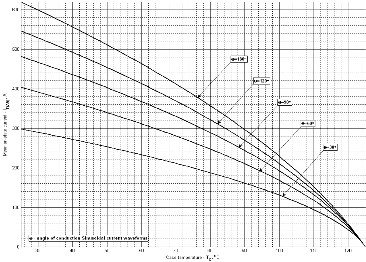
Fig 11 – Maximum case temperature (sinusoidal current waveforms)
