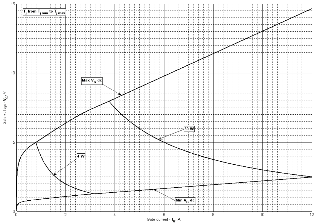
Fig 4 - Gate characteristics – Power curves
