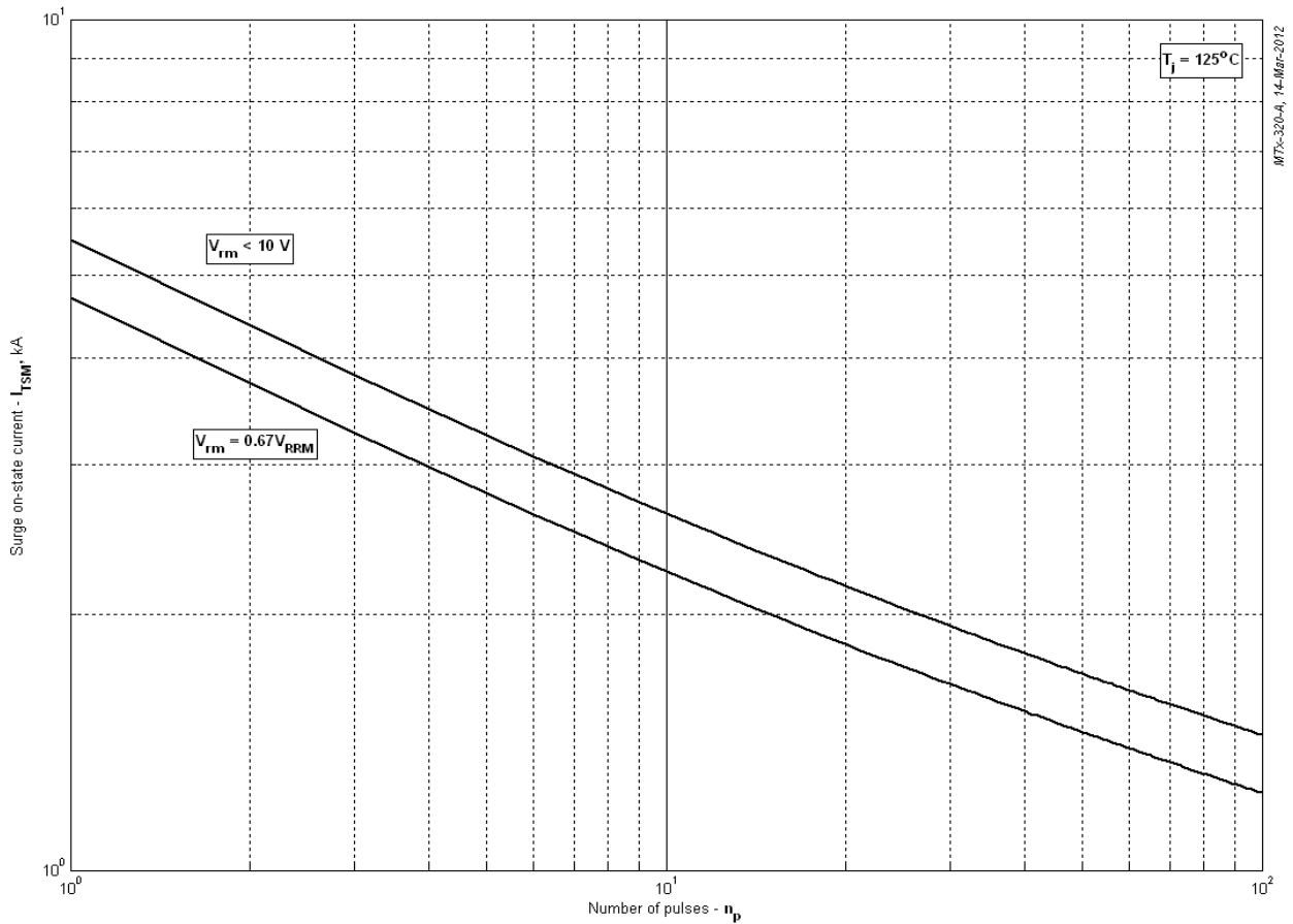
Fig 14 - Maximum surge ratings
