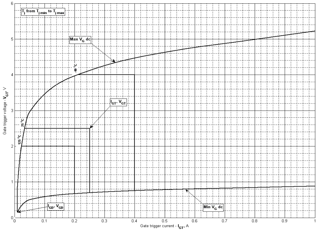
Fig 3 – Gate characteristics – Trigger limits
