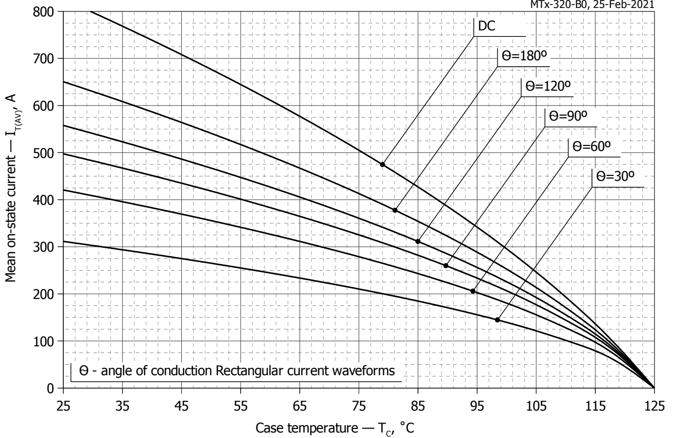
Fig. 9 - Mean on-state current I_{TAV} vs. case temperature T_C for rectangular current waveforms at different conduction angles and for DC ( f=50\text{Hz} , DSC)
