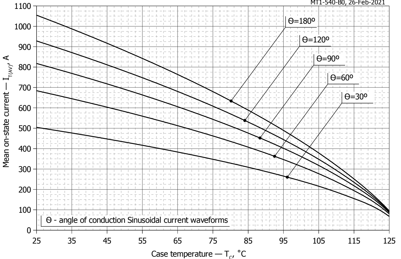
Fig. 8 – Mean on-state current I_{TAV} vs. case temperature T_c for sinusoidal current waveforms at different conduction angles (f=50Hz, DSC)
