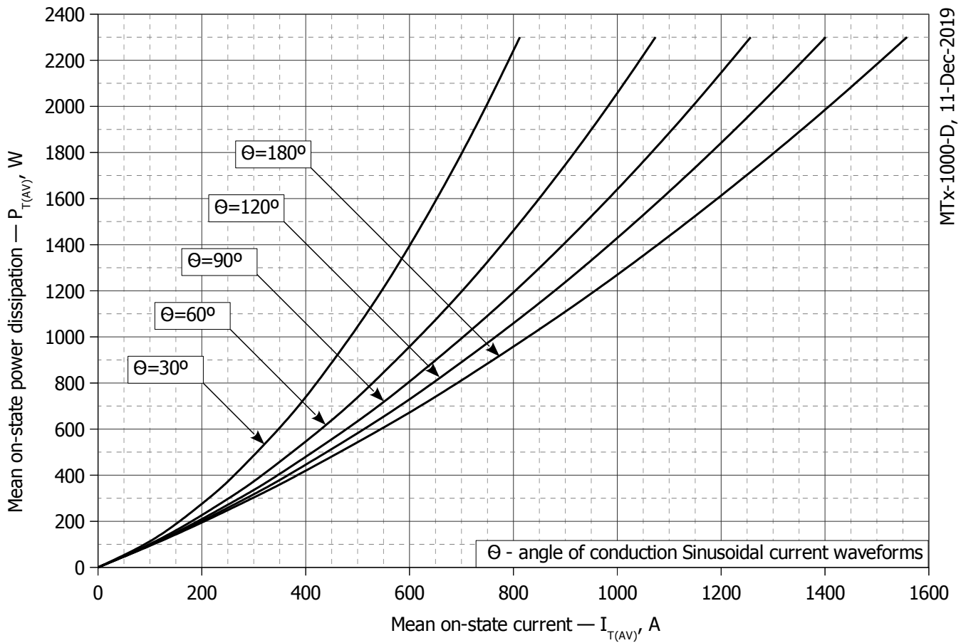
Fig. 9 - Mean on-state power dissipation P_{TAV} vs. mean on-state current I_{TAV} for sinusoidal current waveforms at different conduction angles (f=50Hz, DSC)
