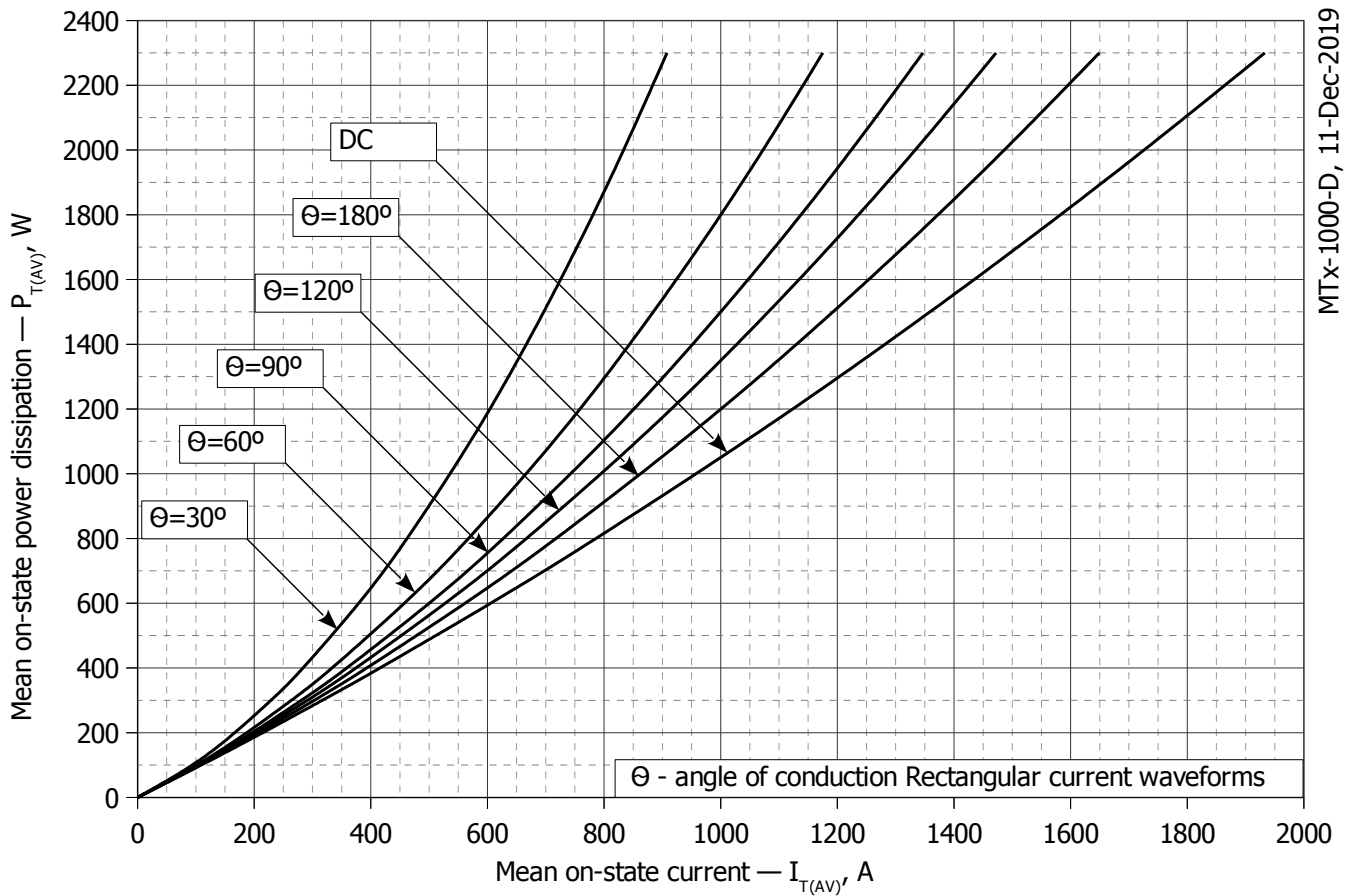
Fig. 10 - Mean on-state power dissipation P_{TAV} vs. mean on-state current I_{TAV} for rectangular current waveforms at different conduction angles and for DC (f=50Hz, DSC)
